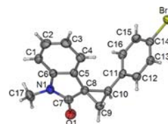
Figure 1. X-ray structure of product 3n .
